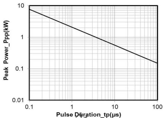
Peak Power vs. Pulse Time
