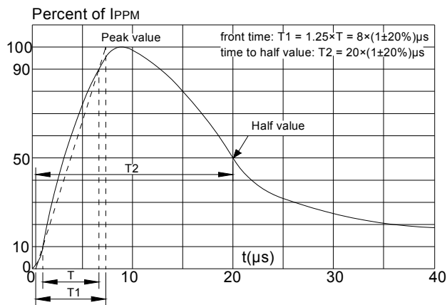
Pulse waveform (8/20μs)
