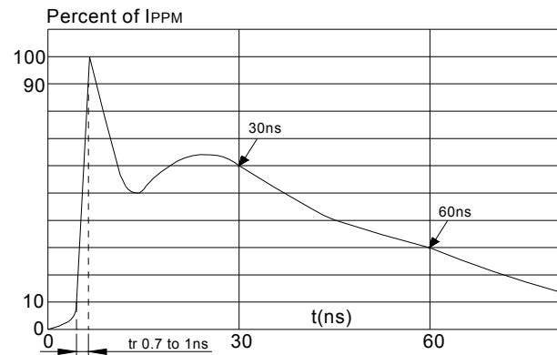
ESD clamping (8KV contact)
